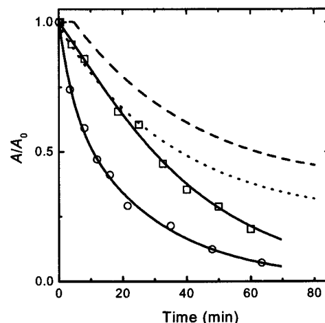
FIGURE 11: Kinetics of thermoinactivation of the \text{NaBH}_4 -reduced form of phosphorylase b at 53 °C (80 mM Hepes-NaOH, pH 6.8). The dotted and dashed lines correspond to thermal inactivation of the native enzyme. Enzyme concentrations were 1.6 mg/mL (circles and dotted line) and 5.2 mg/mL (squares and dashed line).
