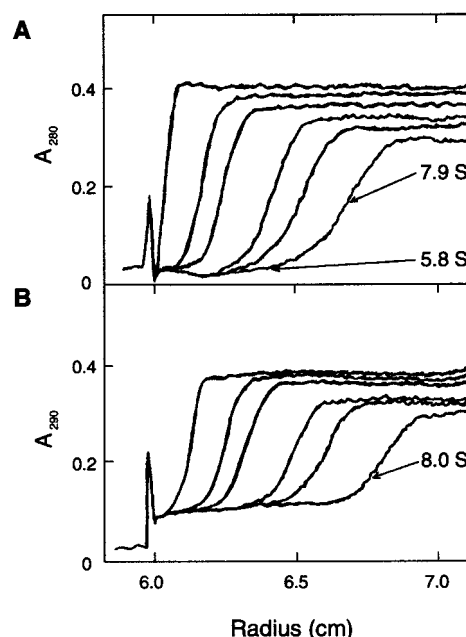
FIGURE 8: Sedimentation velocity patterns of phosphorylase b (0.57 mg/mL) at 49 °C in the absence of AMP (A) and in the presence of 1 mM AMP (B). The rotor speed was 48 000 rpm. The times after attaining the maximum speed were 3, 10, 17, 29, 37, and 50 min (A); 6, 14, 22, 32, 41, and 55 min (B).
