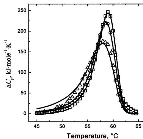
FIGURE 3: Excess heat capacity ( \Delta C_p ) vs temperature profiles for phosphorylase b . Enzyme concentrations were: 0.5 mg/mL (triangles), 3.0 mg/mL (circles), and 6.0 mg/mL (squares). Hepes-KOH, 30 mM, pH 7.0. The scanning rate was 1 °C/min. Solid lines are the best fit simultaneously to all the curves based on model (2).
