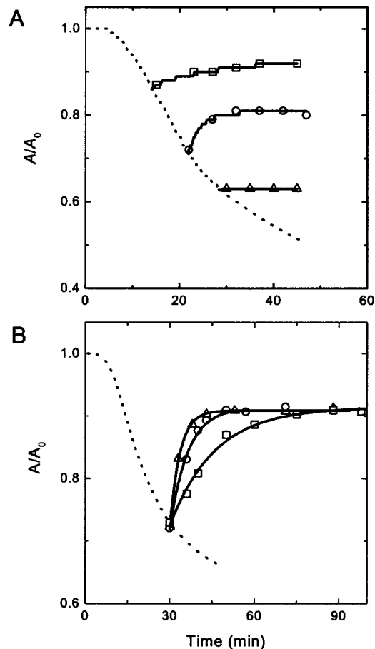
FIGURE 5: Reactivation of phosphorylase b after thermal treatment. (A) Kinetics of reactivation of the enzyme preheated at 53 °C for 15 min (squares), 22 min (circles), and 30 min (triangles). Reactivation was studied at 30 °C. The dotted line corresponds to the thermal inactivation curve of phosphorylase b at 53 °C. Enzyme concentration was 5.2 mg/mL (80 mM Hepes-NaOH, pH 6.8). (B) Effect of the protein concentration on the kinetics of reactivation of phosphorylase b at 30 °C. The enzyme solution (5.2 mg/mL) was preheated at 51 °C for 30 min. Reactivation was carried out at the following enzyme concentrations: 1.3 mg/mL (squares), 2.6 mg/mL (circles), and 5.2 mg/mL (triangles). The dotted line corresponds to the thermal inactivation curve of phosphorylase b (5.2 mg/mL) at 51 °C.
