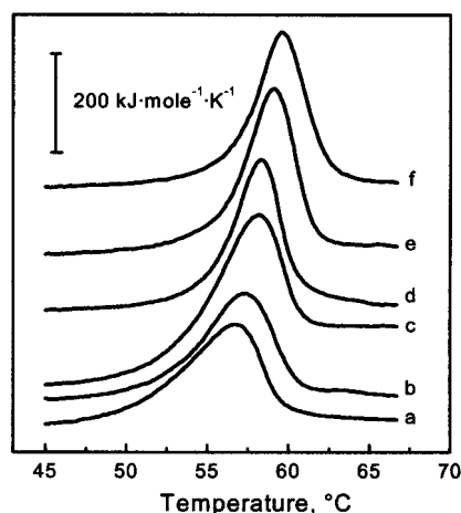
FIGURE 6: Excess heat capacity ( \Delta C_p ) vs temperature profiles for phosphorylase b (5.2 mg/mL) obtained in the absence of specific ligands (a) and in the presence of 20 mM glucose 1-phosphate (b), 3 mM AMP (c), 100 mM glucose (d), 10 mM glucose 6-phosphate (e), or 1 mM FMN (f). 30 mM Hepes-KOH, pH 7.0. The scanning rate was 1 °C/min.
