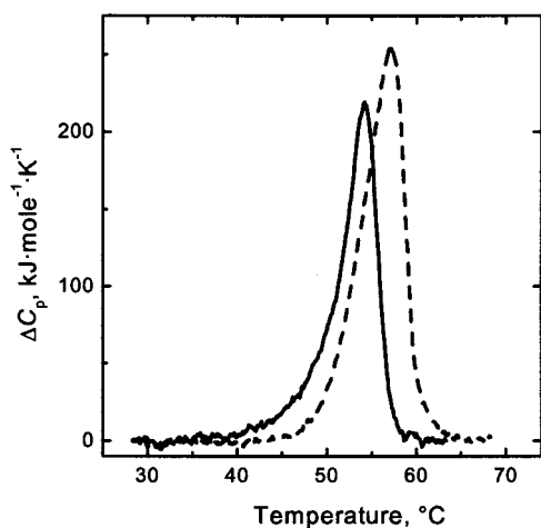
FIGURE 13: Excess heat capacity ( \Delta C_p ) vs temperature profiles for the native (dashed line) and NaBH 4 -reduced (solid line) forms of phosphorylase b . Hepes-KOH, 30 mM, pH 7.0. Enzyme concentration for all the preparations was 1 mg/mL. The scanning rate was 1 ^{\circ}\text{C}/\text{min} .
