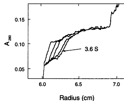
FIGURE 12: Sedimentation velocity pattern vs. of \text{NaBH}_4 -reduced form of phosphorylase b (0.92 mg/mL) at 53 °C. The rotor speed was 48 000 rpm. The times of sedimentation were 26, 33, 38, 51, and 54 min.
