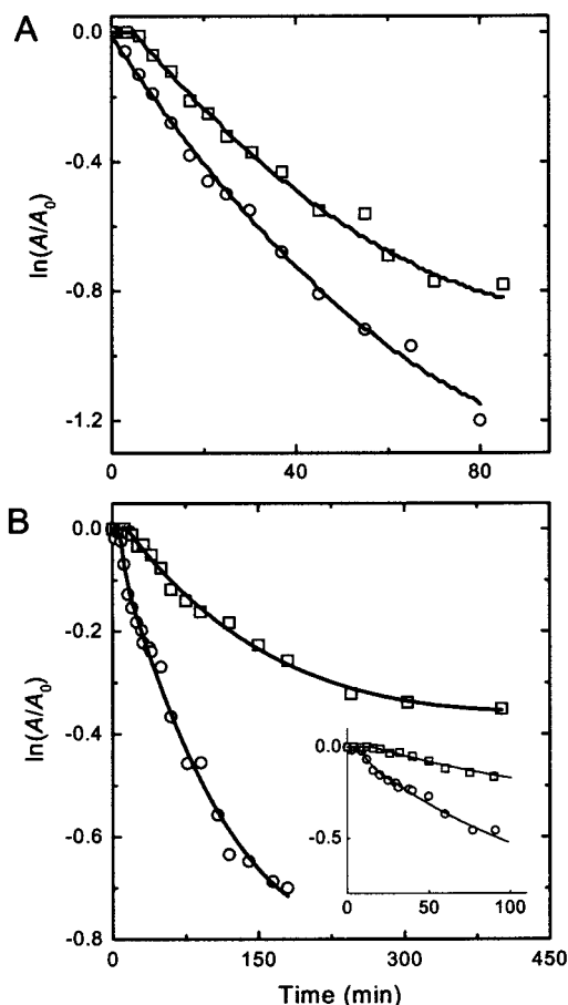
FIGURE 2: Kinetics of thermal inactivation of phosphorylase b at 53 °C (A) and 51 °C (B) in semilogarithmic coordinates (80 mM Hepes-NaOH, pH 6.8). A/A_0 is the relative enzymatic activity, t is time. Enzyme concentrations are 1.6 mg/mL (circles) and 5.2 mg/mL (squares). Insert in panel B shows the initial parts of the kinetic curves (the axes are identical with those for the main figure).
