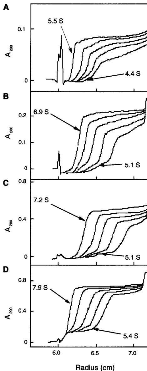
FIGURE 4: Sedimentation of phosphorylase b at 53 °C (80 mM Hepes-NaOH, pH 6.8). Enzyme concentration: (A) 0.03; (B) 0.46; (C) 0.92, and (D) 2.5 mg/mL. Time after reaching 60 000 rpm: (A) 6, 14, 20, 25, and 33 min; (B) 10, 15, 21, 27, and 34 min; (C) 12, 18, 23, 29, and 36 min; (D) 7, 13, 18, 22, and 27 min. Ordinate axes show optical density at 280 or 290 nm.
