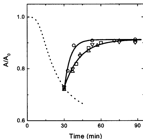
FIGURE 9: Effect of 2 mM FMN (○), 1.8 mM AMP (▽), and 3 mM glucose 6-phosphate (△) on the kinetics of reactivation of phosphorylase b (1.3 mg/mL) preheated at 51 °C for 30 min. Squares correspond to reactivation in the absence of ligands. Reactivation was studied at 30 °C. The dotted line is the thermal inactivation curve of phosphorylase b (5.2 mg/mL) at 51 °C. When studying reactivation, the preheated enzyme solution was diluted to 1.3 mg/mL.
