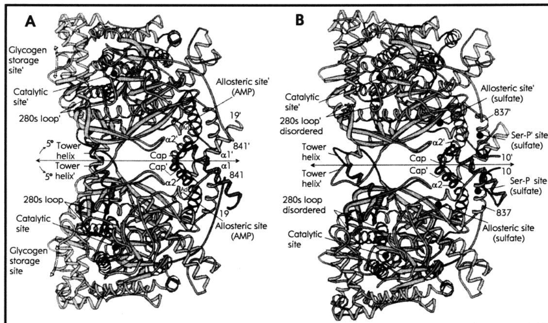
FIGURE 1: Ribbon representation of the structure of T (A) and R (B) states of muscle phosphorylase b dimer viewed perpendicular to the molecular dyad axis [Reprinted with permission from Barford, D., and Johnson, L. N. (15)].
