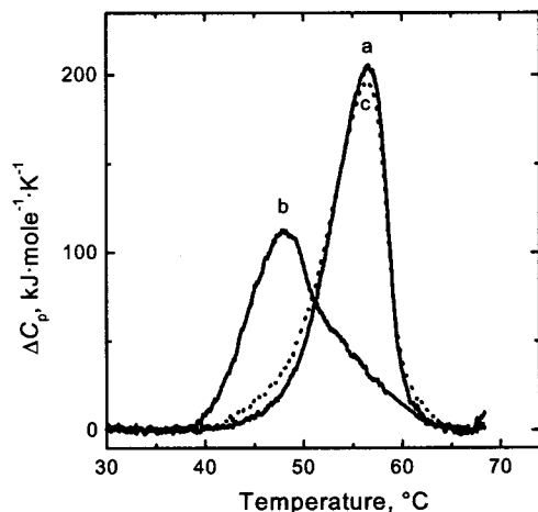
FIGURE 10: Excess heat capacity ( \Delta C_p ) vs temperature profiles for holoform (a), apoform (b), and reconstituted form (c) of phosphorylase b (30 mM Hepes-KOH, pH 7.0). Enzyme concentration was 0.7 mg/mL for all the enzyme preparations. The scanning rate was 1 °C/min.
