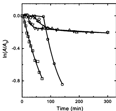
FIGURE 7: Effect of 2 mM FMN (○), 1.8 mM AMP (▽), and 3 mM glucose 6-phosphate (Δ) on the kinetics of thermal inactivation of phosphorylase b (5.2 mg/mL; 53 °C). Squares correspond to thermoinactivation of the enzyme without any additions. The data are presented in semilogarithmic coordinates. Hepes-NaOH, 80 mM, pH 6.8.
